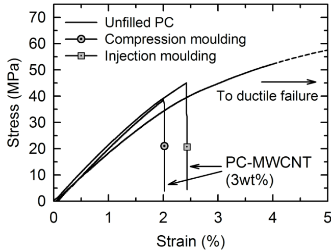
FIGURE 8 Representative stress-strain curves of compression moulded and injection moulded PC-MWCNT 2205 and unfilled compression moulded PC 2205.
