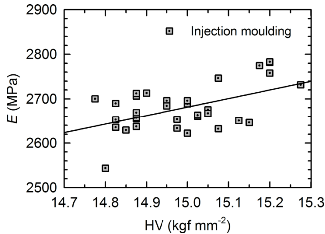
FIGURE 10 Relationship between Young's modulus and surface hardness for injection moulded specimens, with linear regression, giving a correlation coefficient R = 0.52
